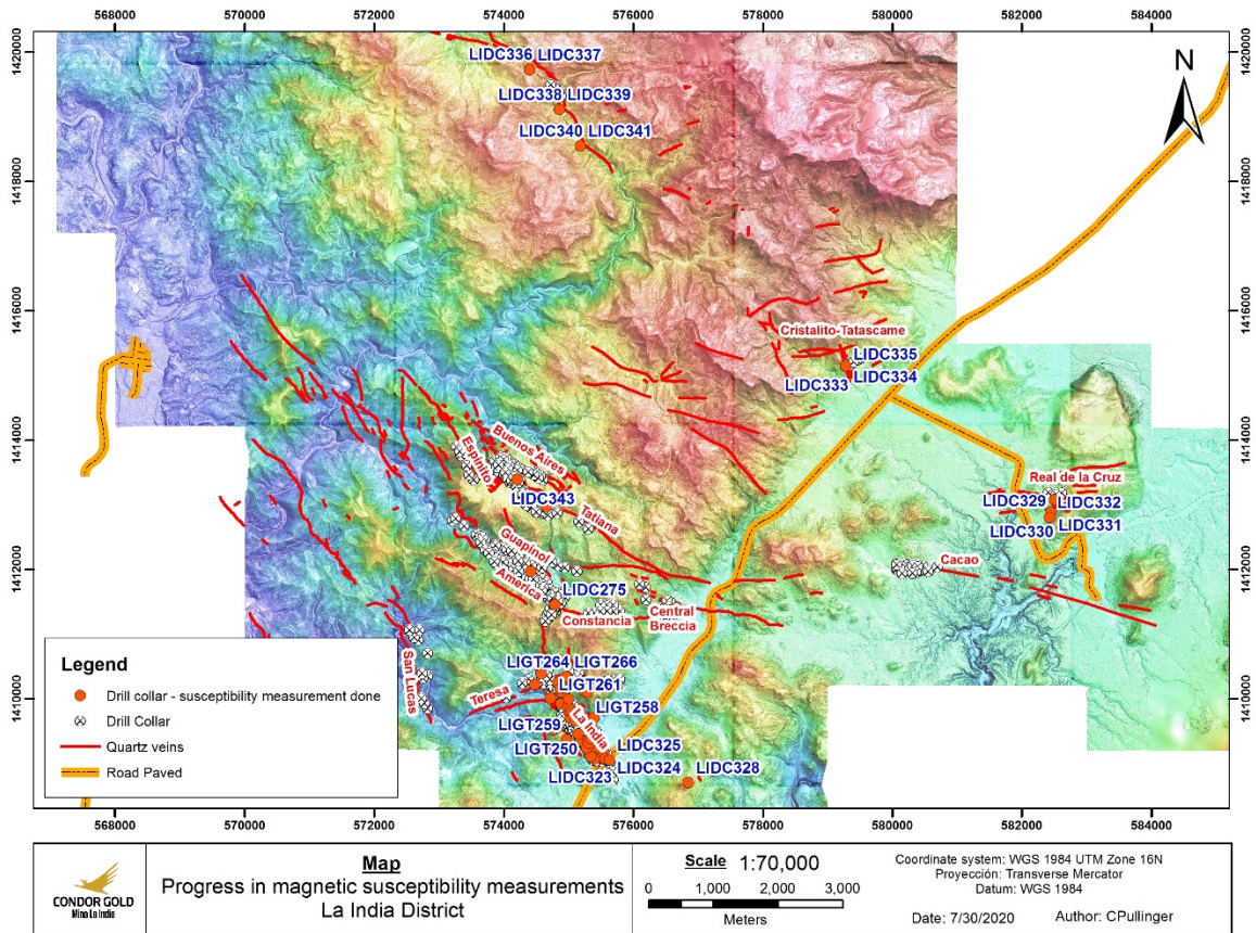
Figure 1. Map showing drill holes (in blue) with magnetic susceptibility measurements.
